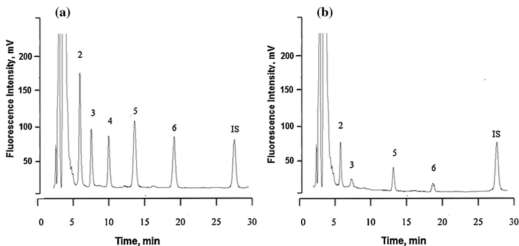
Fig. 5. Representative chromatograms of (a) spiked serum sample with aldehydes (5 nM each) and (b) serum of healthy human, peaks 2–6 as in Fig. 3.
