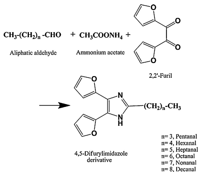
Fig. 2. The reaction scheme for fluorogenic derivatization of saturated aliphatic aldehydes with 2,2'-furil.
