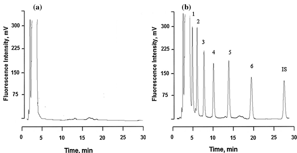
Fig. 3. Chromatograms obtained from (a) reagent blank and (b) standard solution mixture of aldehydes (5 nM each) after derivatization. Peaks: 1 = pentanal, 2 = hexanal, 3 = heptanal, 4 = octanal, 5 = nonanal and 6 = decanal.
