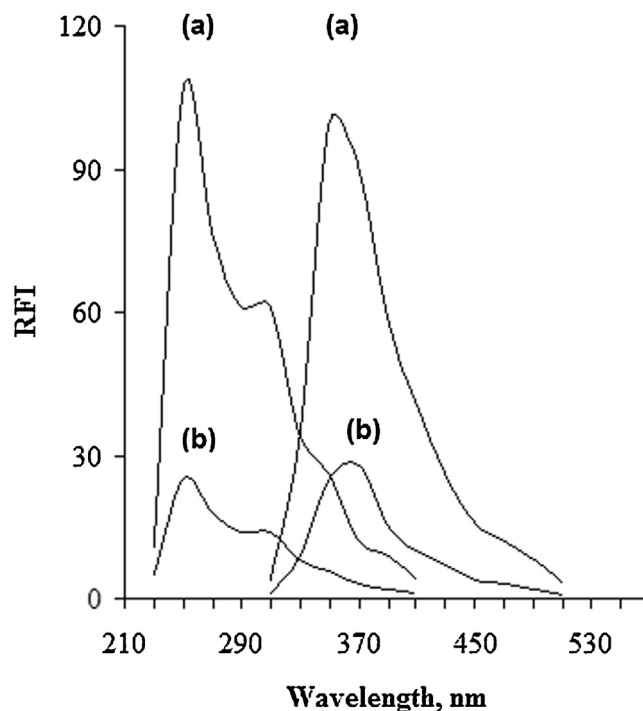
Fig. 1. Excitation and emission spectra of (a) derivatized decanal (200 nM) and (b) reagent blank at excitation and emission maxima at 250 nm and 355 nm, respectively.
