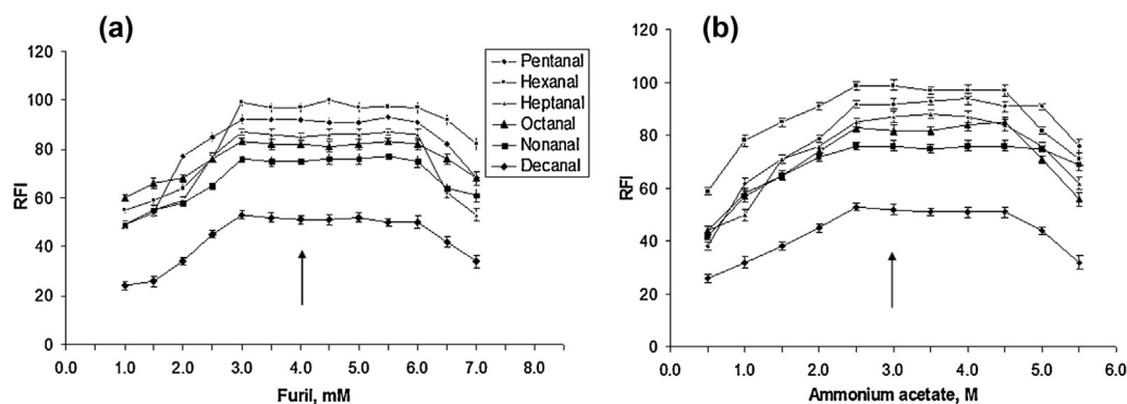
Fig. 4. Optimization conditions of derivatization reaction of standard mixture of studied aldehydes (5 nM each): effects of (a) 2,2'-fural concentration, and (b) ammonium acetate concentration on fluorescence intensity. The data represent error bars of three determinations.
